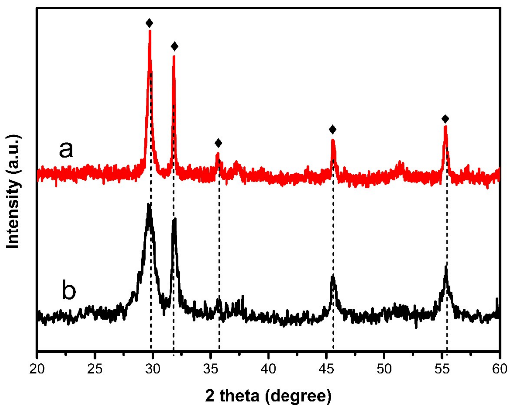
Fig. S1. XRD patterns of (a) before and (b) after the photocatalytic reaction of \text{PONs}_{(1/3)} .
