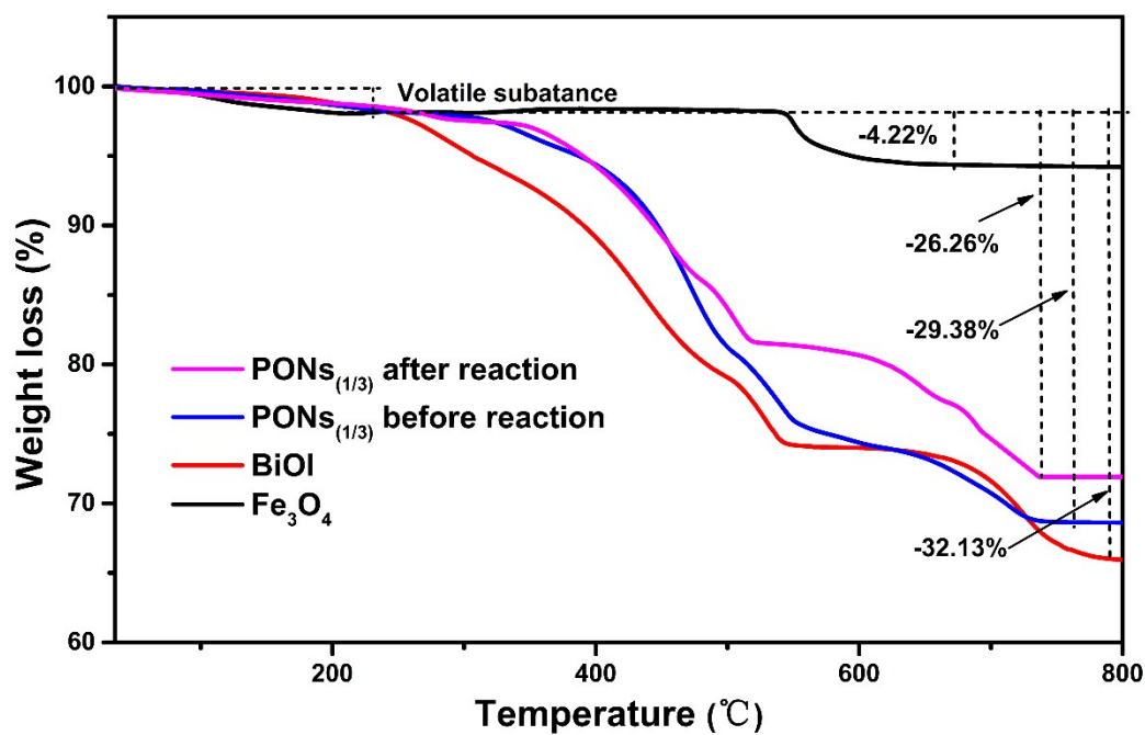
Fig. S2. TG curves of as-prepared BiOI, Fe 3 O 4 , before and after photocatalytic reaction of PONs (1/3) , respectively.
