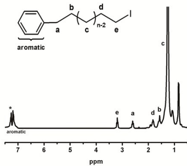
Figure. s2 ^1\text{H} NMR spectrum of PM-I in \text{C}_6\text{D}_4\text{Cl}_2
