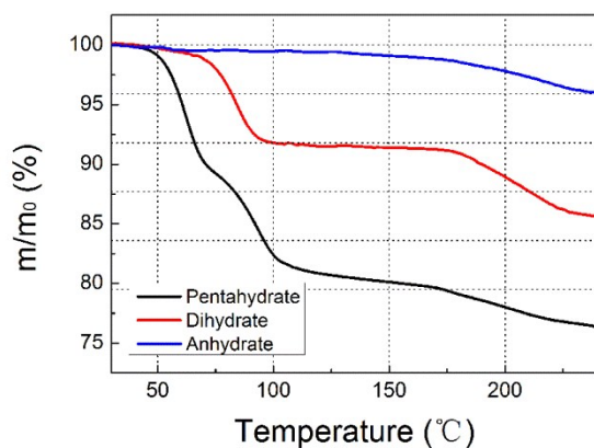
Fig. S2. TGA traces of MB pentahydrate, dihydrate and anhydrate.
