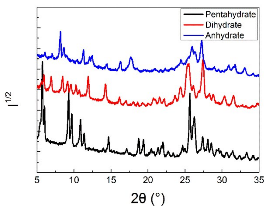
Fig. S1. XRPD patterns of the MB pentahydrate, dihydrate and anhydrate, measured with Cu K α radiation.
