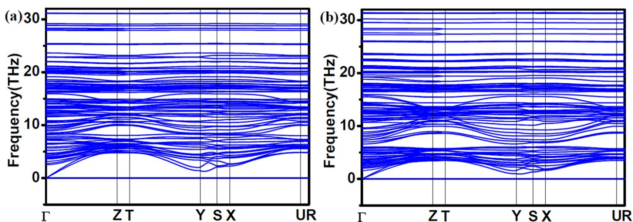
Fig. S1 Phonon dispersion curves for (a) \text{Ru}_2\text{B}_7 and (b) \text{Os}_2\text{B}_7 .
