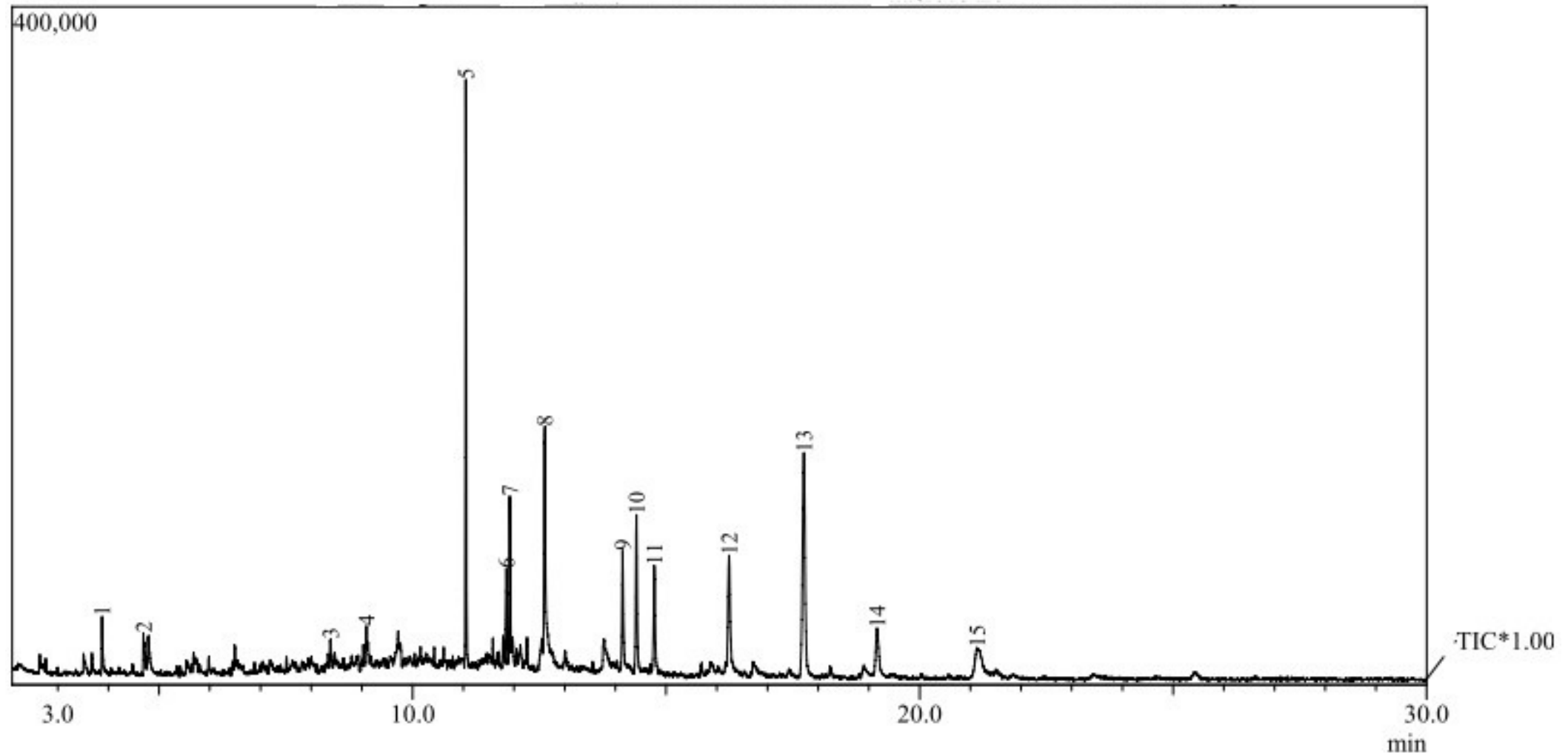
Fig.S3. Total ion chromatograms of biocrude obtained with Kaoline catalyst
