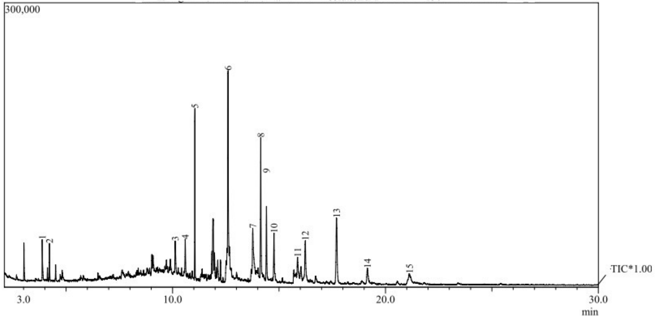
Fig.S4. Total ion chromatograms of biocrude obtained with Dolomitic limestone catalyst
