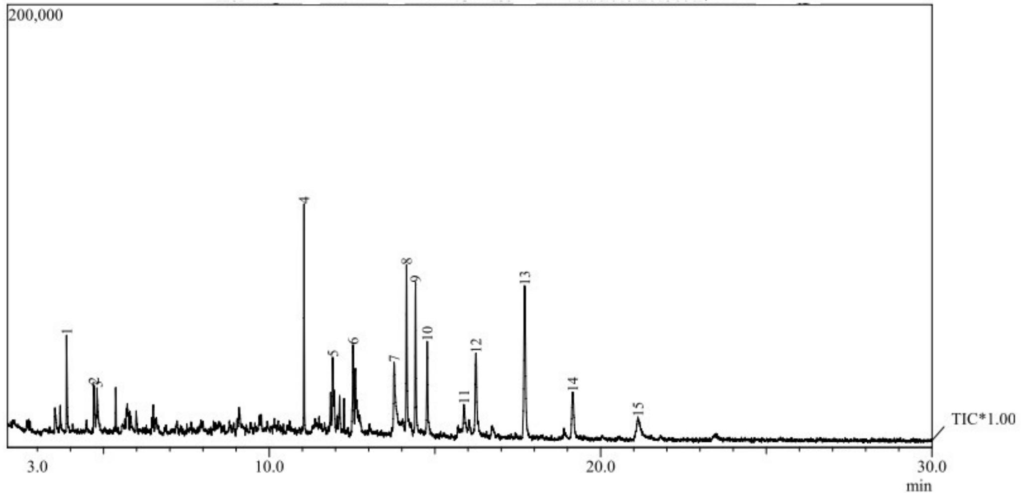
Fig.S2. Total ion chromatograms of biocrude obtained with Montmorillonite catalyst
