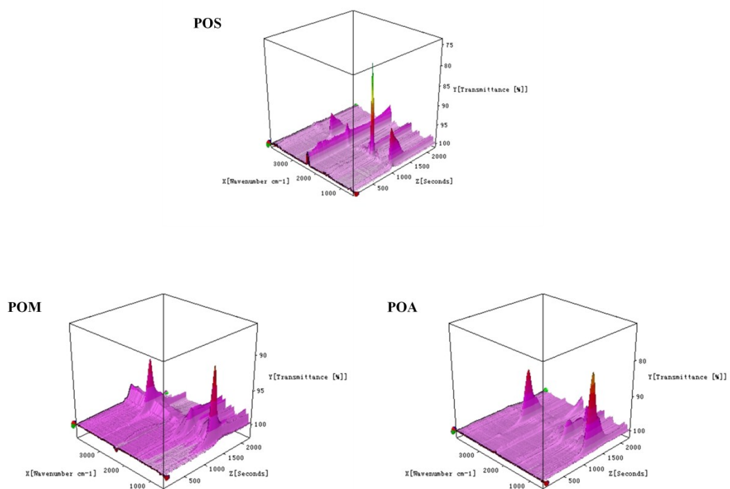
SI Fig. 1. TGA-FTIR 3D spectra of pyrolysis gases during thermal degradation of POS, POM and POA.
