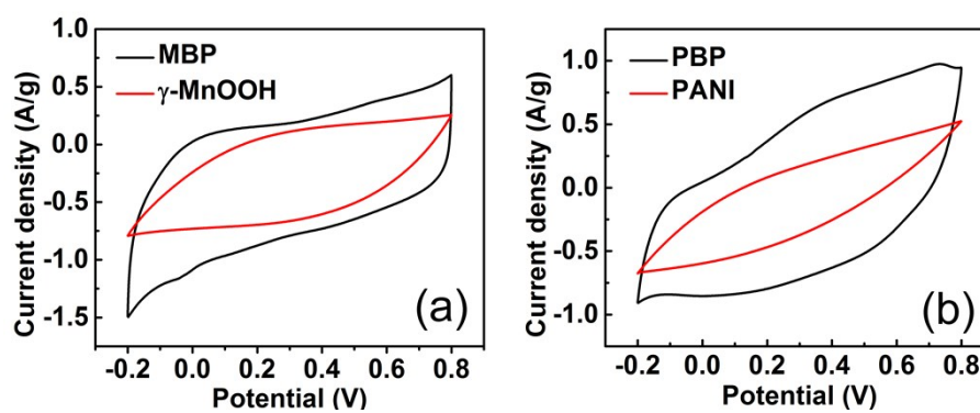
Fig. S4. The CV curves of (a) MBP and \gamma -MnOOH (b) PBP and PANI at the current density of 5 \text{ mV s}^{-1}
