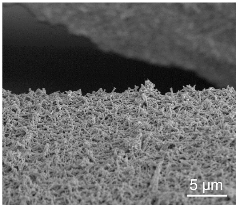
Fig. S2. The cross-sectional view of PMBP
