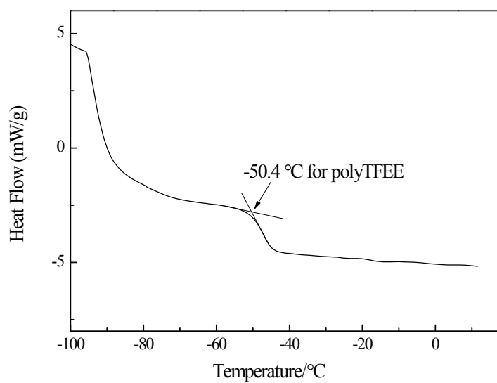
Fig.S1 DSC cruve of polyTFEE
