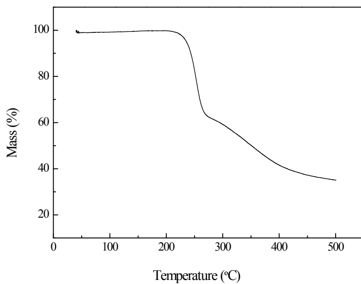
Fig.S4 TGA cruve of sampe GAP.
