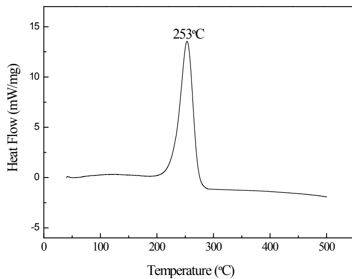
Fig.S3 DSC cruve of sampe GAP.
