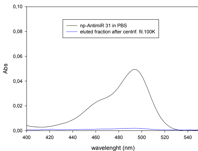
Fig S1. UV-vis absorption spectra of NG-AntimiR-31 IC and its eluted fraction after incubation for 24 h in isotonic PBS at 37°C and centrifuge filtration (MWCO 100 kDa).
