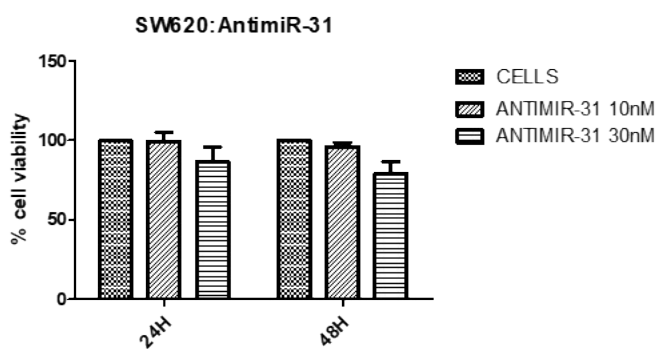
Fig S2. Results of cell viability of SW620 cells treated with different concentrations of AntimiR.
