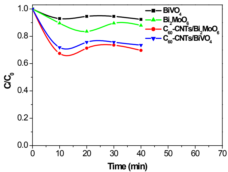
Fig. S1 The degradation curves of Rh B over different catalysts without visible light irradiation.
