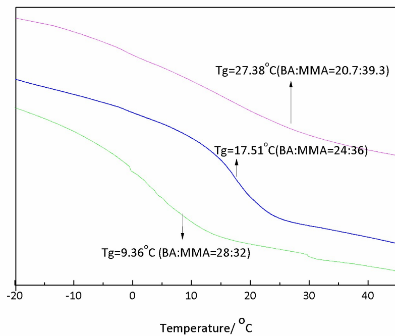
Fig.S1. DSC thermograms of latex particle with different weight ratio BA/MMA
