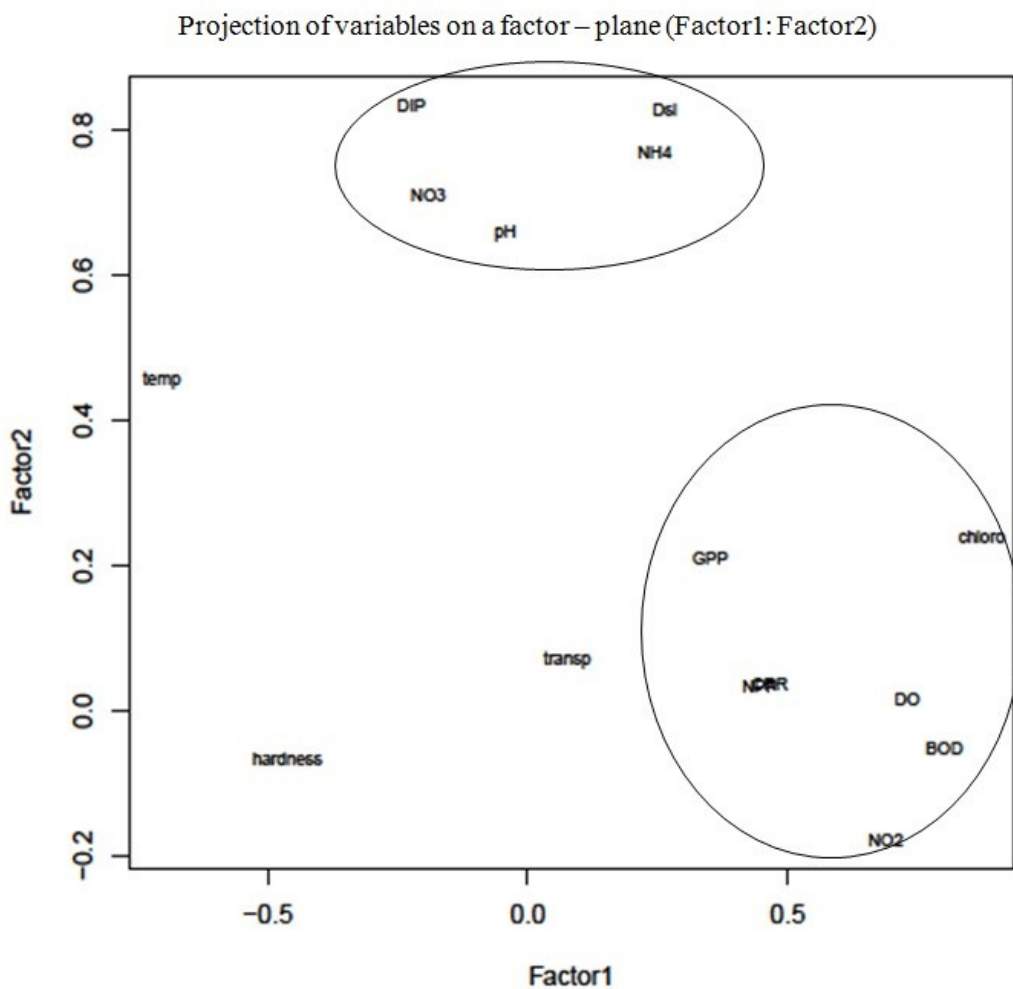
Supplementary figure 1: Factor analysis (FA) plot of factor 1 vs. factor 2 for environmental variables recorded from the study area during the entire study period
