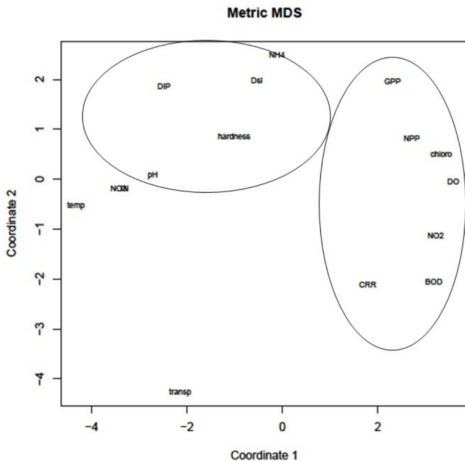
Supplementary figure 2: Metric multidimensional scaling (MDS) plot of Coordinate 1 vs. Coordinate 2 for environmental variables recorded from the study area during the entire study period
