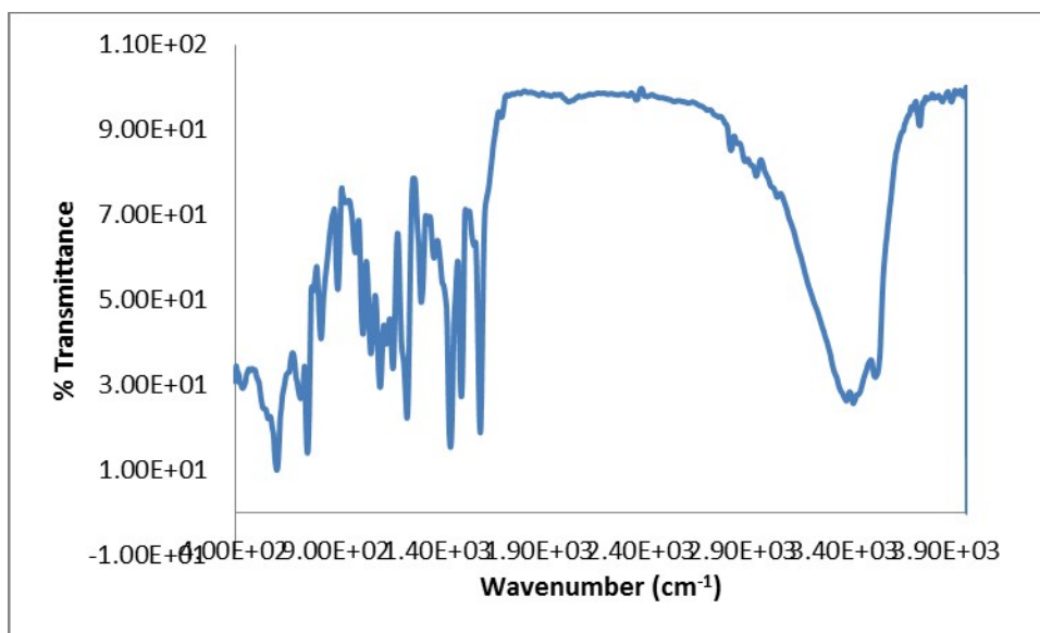
Figure SI 1(a): FTIR spectral peaks of complex 6
