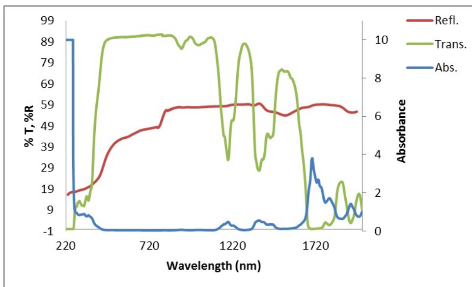
Figure SI 2(b): Absorbance, Transmittance and Reflectance spectra of complex 6
