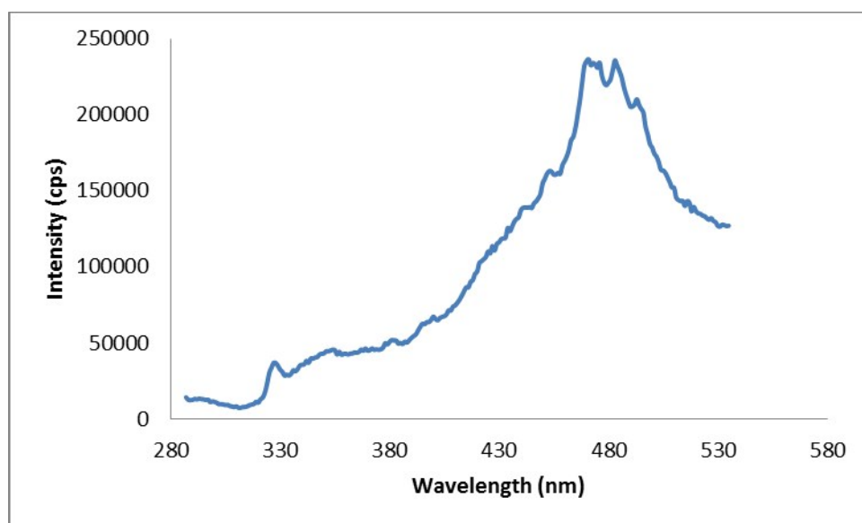
Figure SI 3(a): Solid state fluorescence spectra of complex 2
