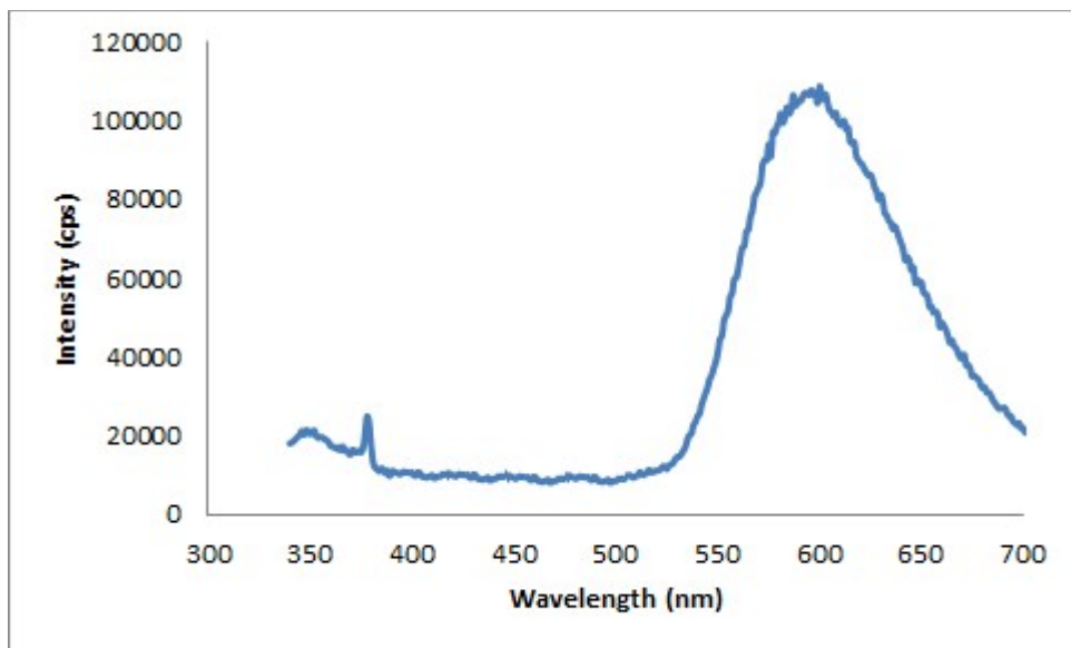
Figure SI 3(b): Solid state fluorescence spectra of complex 6
