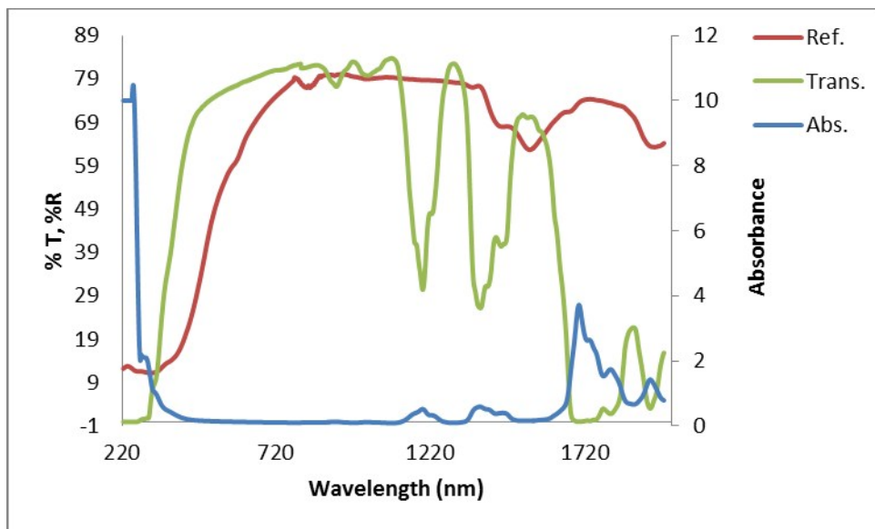
Figure SI 2(a): Absorbance, Transmittance and Reflectance spectra of complex 1
