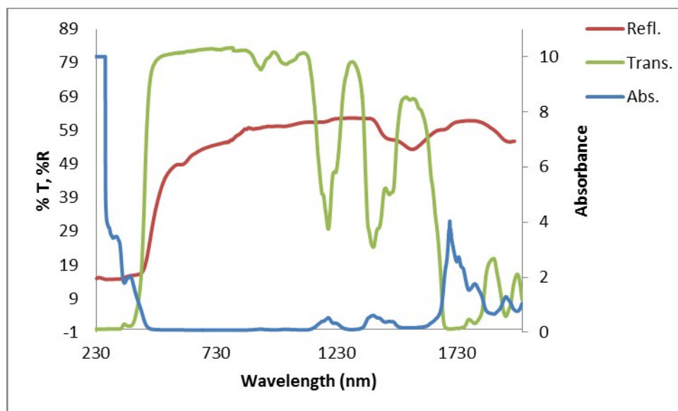
Figure SI 2(c): Absorbance, Transmittance and Reflectance spectra of complex 10
