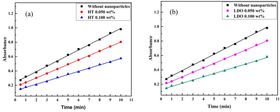
Fig. S1. Effect of nanoparticles concentration on the diffusion of MPD to hexane: (a) HT; (b) LDO
