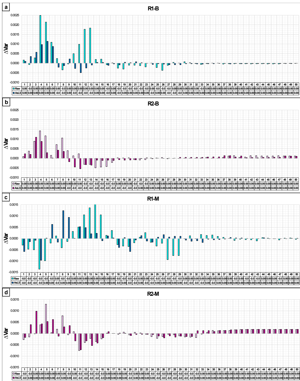
Supplementary Fig. 1 Variance differences of PLS1-DA models against the respective PLS2-DA models that constructed using the raw and AsLS datasets and plotted by the first 50 PLS components. The variances were estimated via 10-fold CV.
