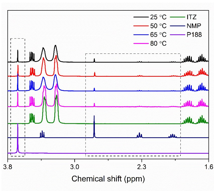
Fig.S1 NMR spectrum of ITZ precipitated at different precipitation temperatures.
