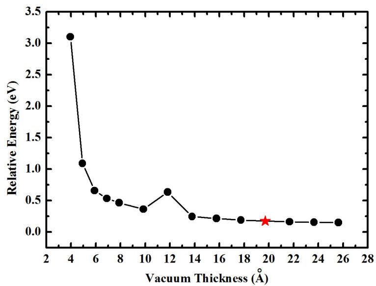
Figure S1. The relative energy of the electron-doping (0.1 e/cell) \beta_0 -PC vs. the vacuum thickness. The red star stands for the vacuum thickness used in our calculations of the superconductivity and other related properties.
