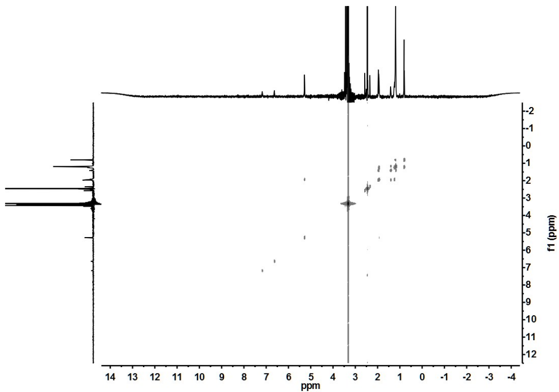
Fig. S1 2D ^1\text{H} NMR spectra of EP
