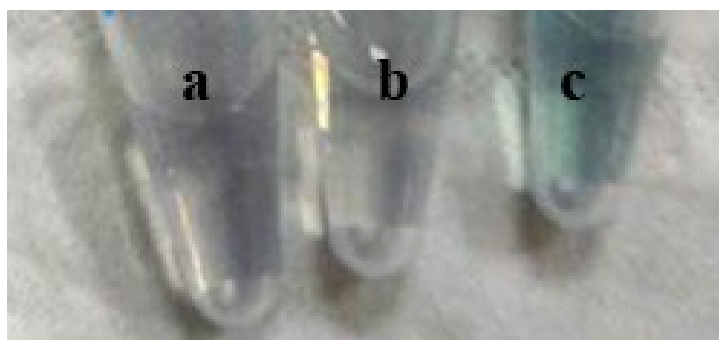
Fig S1. The photos of color (a) in the presence of 12.5 \mu\text{M} D-Cys, (b) in the presence of 12.5 \mu\text{M} L-Cys (c) GNRs. \text{Cu}^{2+} : 0.125 mM.
