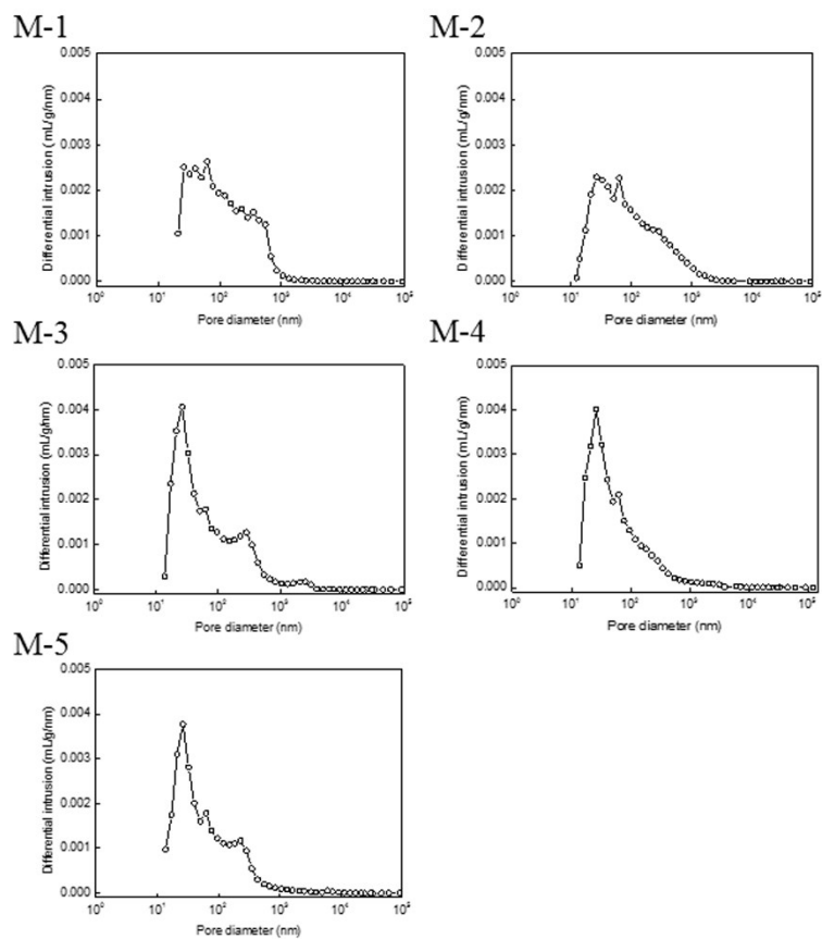
Fig. S1 The pore size distribution of the membranes.
