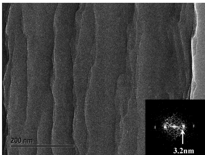
Figure S1. Cross-sectional high resolution TEM image of large area self-assembled PCBDANI film.
