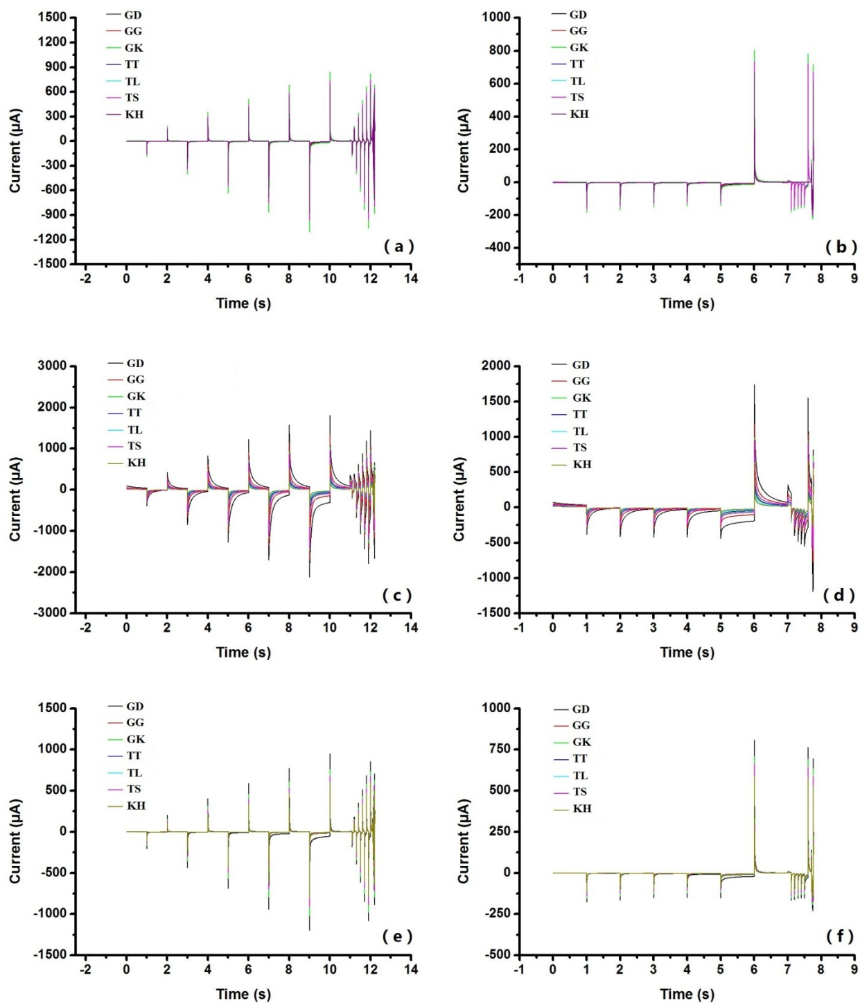
Fig. S1 The response current curves of modified electrodes array to 7 brands of rice wines.
