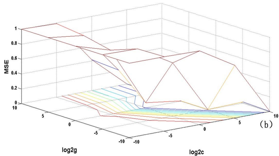
Fig. S3 The variation trend of the accuracy rate of ELM model (a) and the 3D view of parameter selections of LIBSVM (b).
