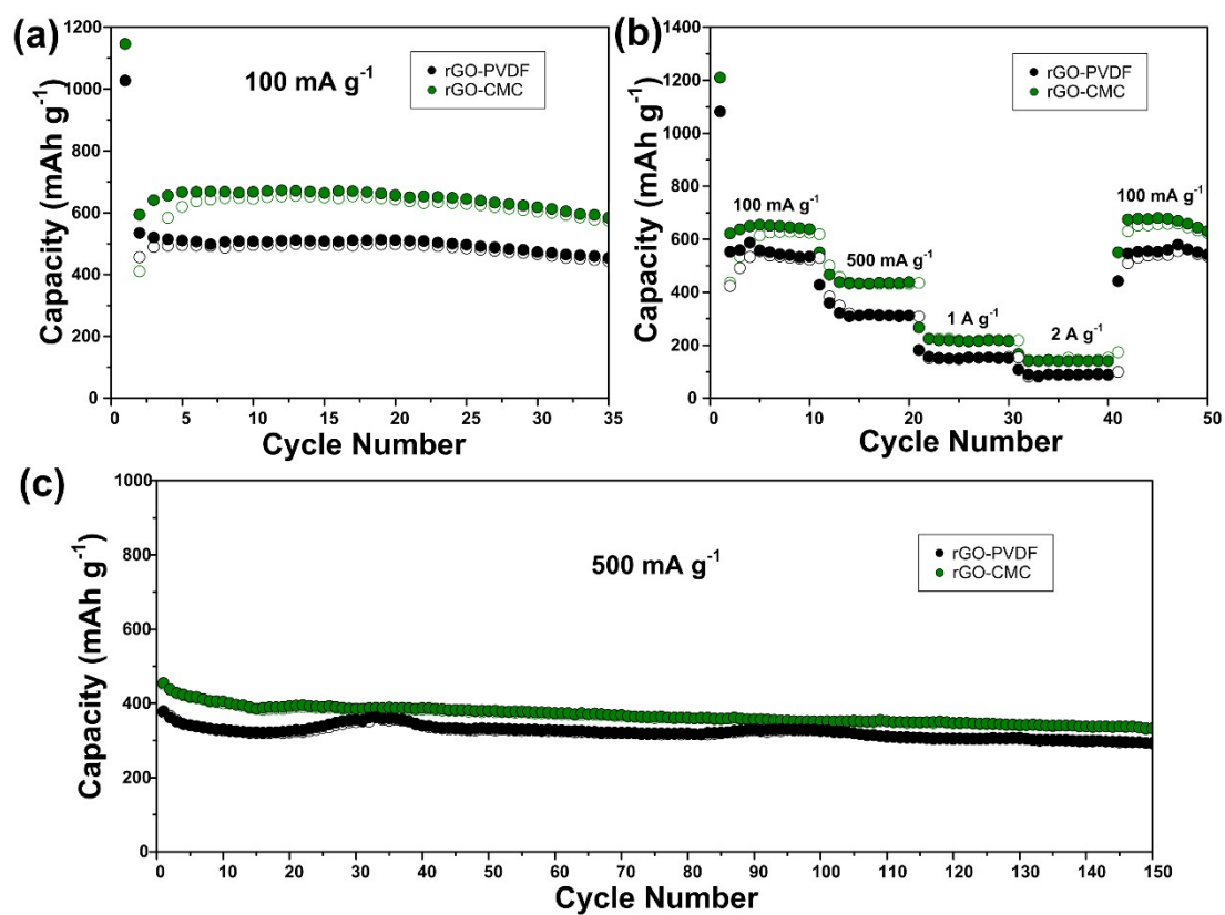
Fig. S2 (a) Cycling performance and (b) rate capability of rGO-PVDF and rGO-CMC. (c) Continuous long-term cycling performance of rGO-PVDF and rGO-CMC after the rate test.
