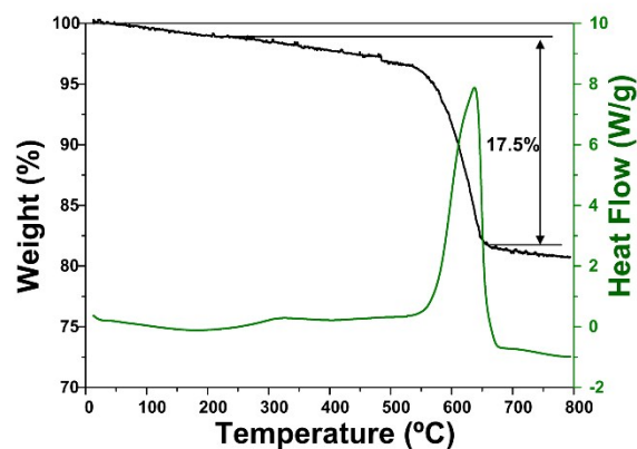
Fig. S1 TGA and DSC curves of ZS.
