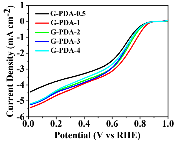
Fig.S2. LSV curves at 1600rpm for the G-PDA-m samples.
