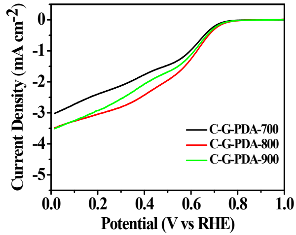
Fig.S1. LSV curves at 1600rpm for C-G-PDA-t samples.
