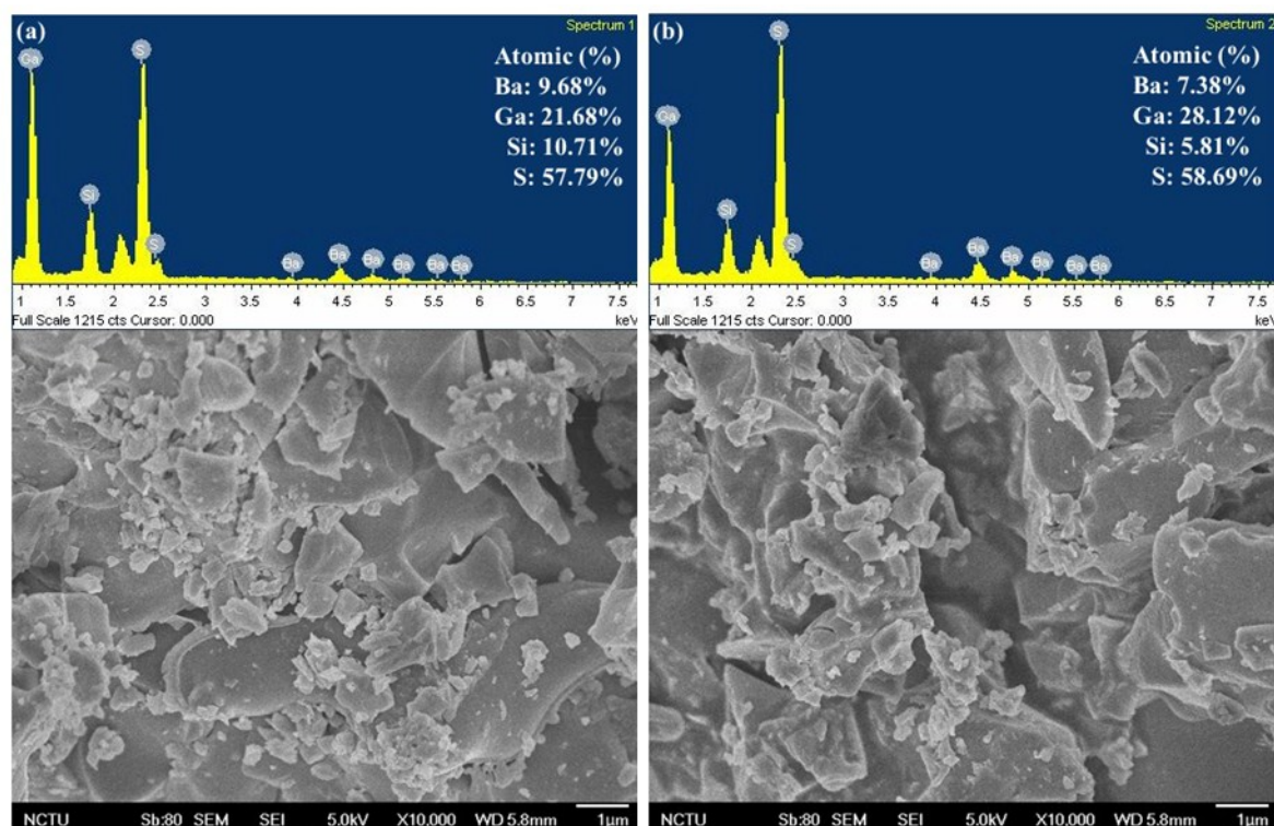
Figure S1. EDS spectra and SEM image of as-synthesized (a) \text{BaGa}_2\text{SiS}_6 and (b) \text{Ba}_2\text{Ga}_8\text{SiS}_{16} phosphor.
