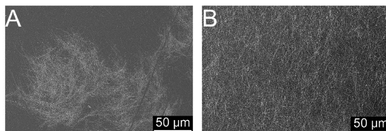
Figure S1 TCE fabricated with AgNW ink without HPMC (A) and with HPMC (B).
