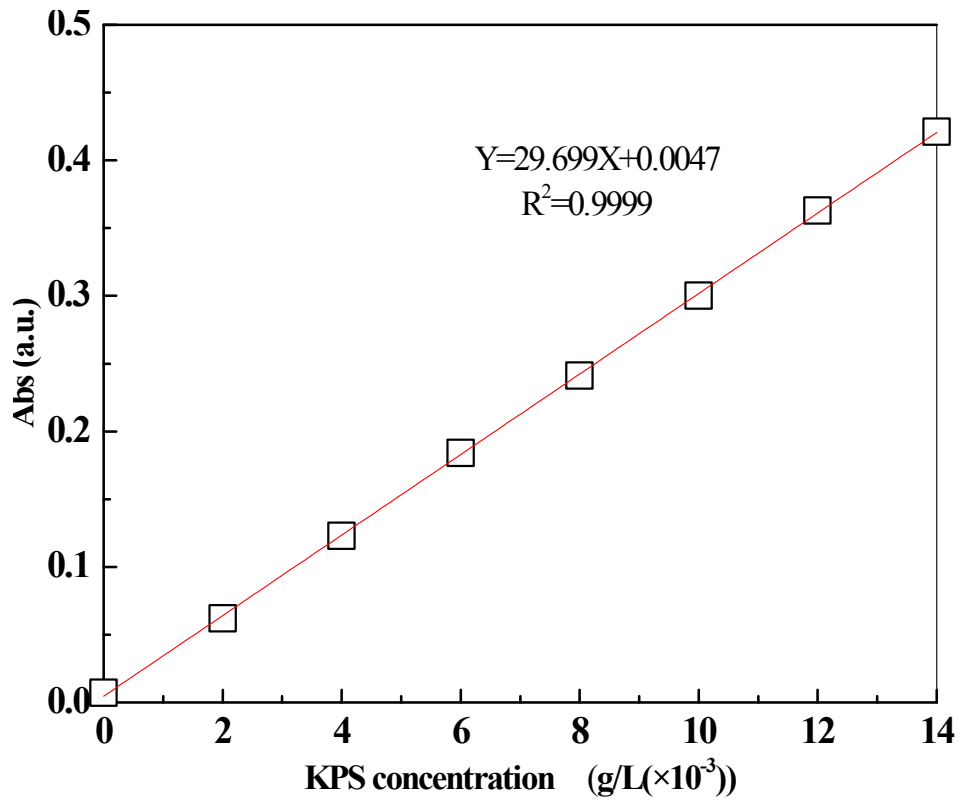
Fig. SM-1 Persulfate concentration standard curve
