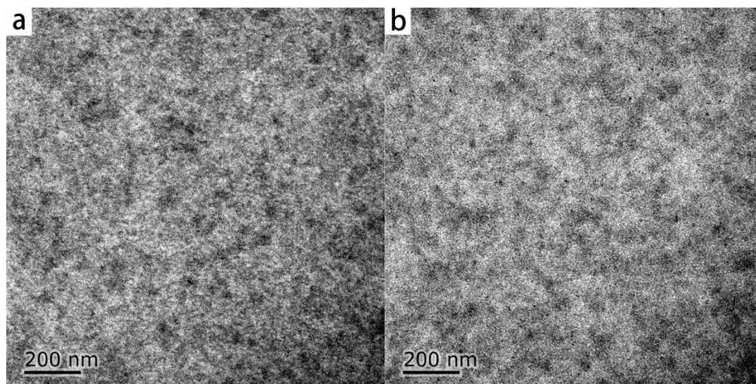
Figure S1 TEM images of PTB7:PC 71 BM blend films (a) without PbS QDs doped, (b) with 5% PbS QDs doped.
