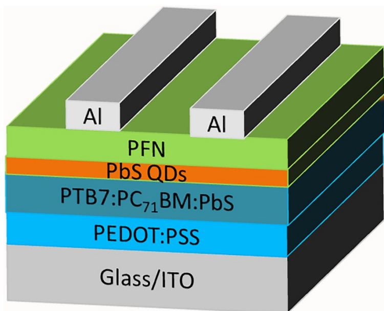
Figure S2 Schematic image of polymer BHJ solar cells device with structure of ITO/PEDOT:PSS/PTB7:PC 71 BM/PbS QDs/Al.
