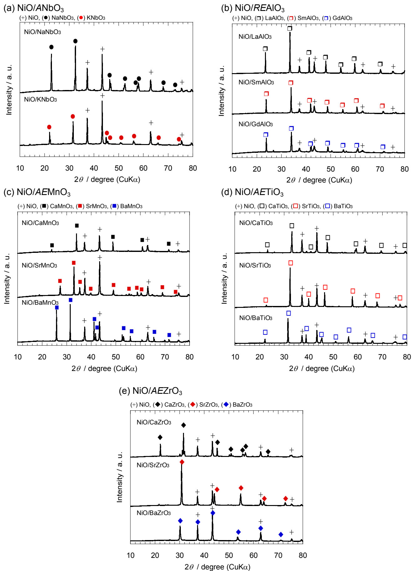
Fig. S1 XRD patterns of 40 wt.% (a) NiO/ANbO 3 , (b) NiO/REAlO 3 , (c) NiO/AEMnO 3 , (d) NiO/AETiO 3 , and (e) NiO/AEZrO 3 after calcination at 600 °C.
