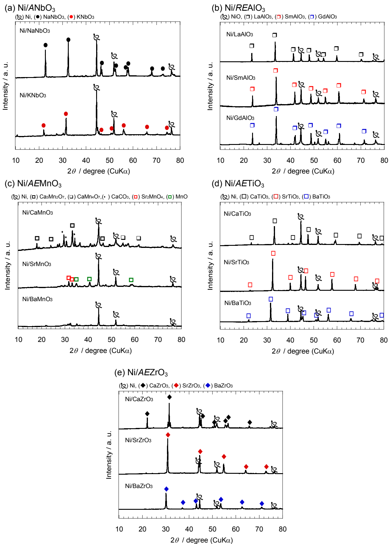
Fig. S2 XRD patterns of 40 wt.% Ni/ANbO 3 , Ni/REAlO 3 , Ni/AEMnO 3 , Ni/AETiO 3 , and Ni/AEZrO 3 after reduction at 600 °C.
