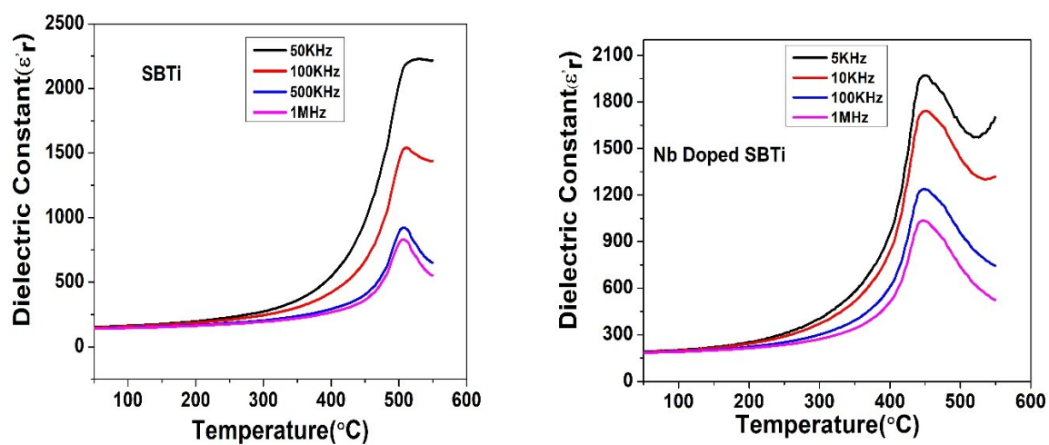
Figure: Dielectric constant versus temperature at different frequencies.
