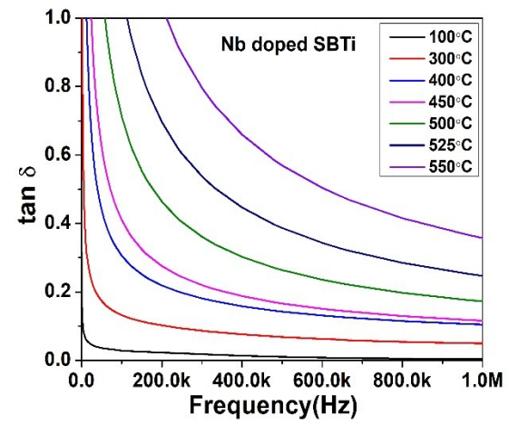
Figure: Frequency response of dielectric loss ( \tan \delta ) at different temperatures.
