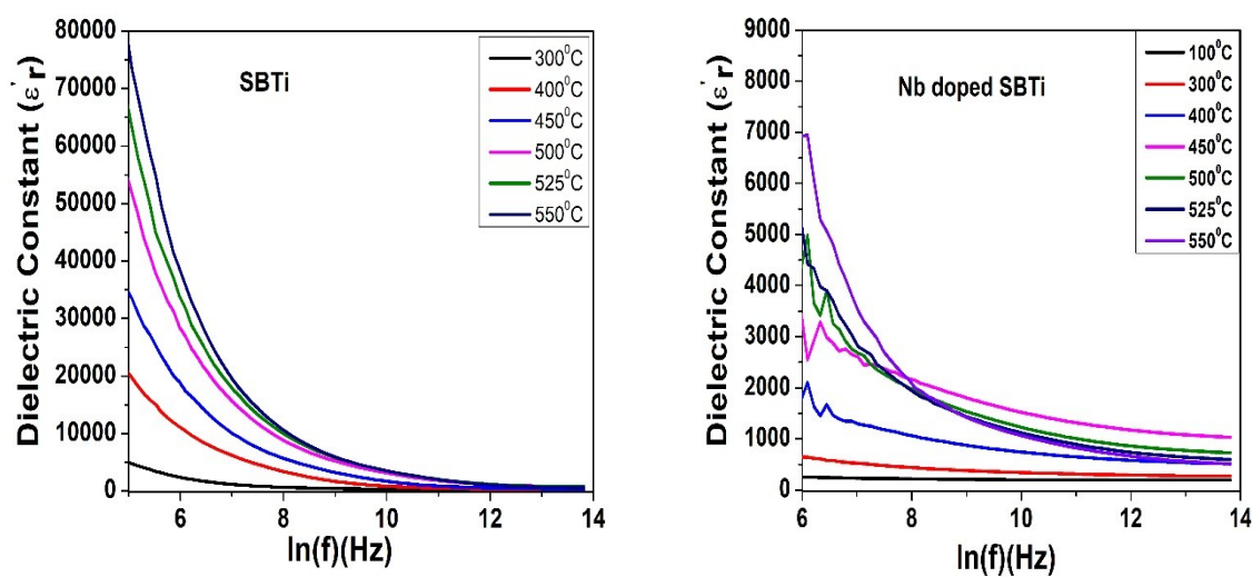
Figure: Frequency response of dielectric constant at different temperatures.
