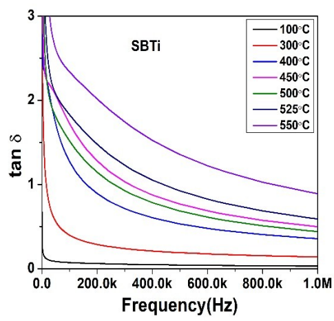
Figure: Frequency response of dielectric loss ( \tan \delta ) at different temperatures.
