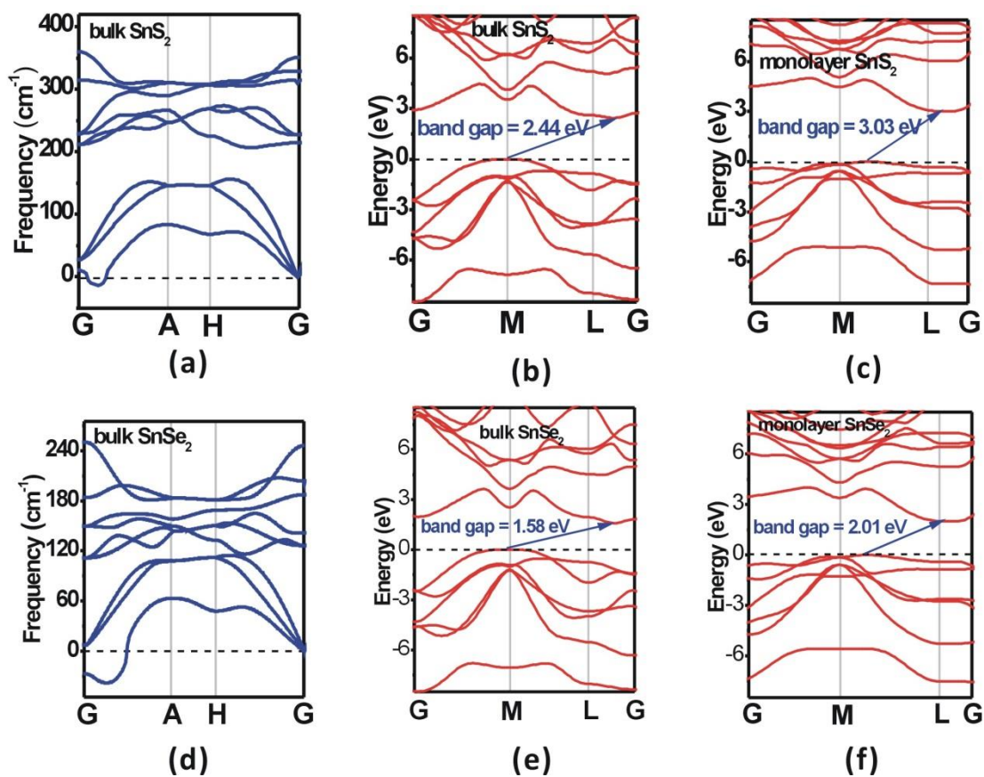
Figure S1. The phonon spectra of bulk (a) SnS 2 and (d) SnSe 2 , (b), (c), (e) and (f) are the band structure of bulk phase and monolayers at the HSE06 level.
