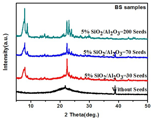
Fig. S1 The XRD patterns of the BS samples with the seeds with different SiO 2 /Al 2 O 3 ratios.
