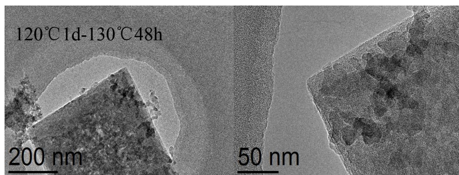
Fig.S2 TEM images of BS-2 sample obtained after crystallization (120°C 1d-130°C 2d).
