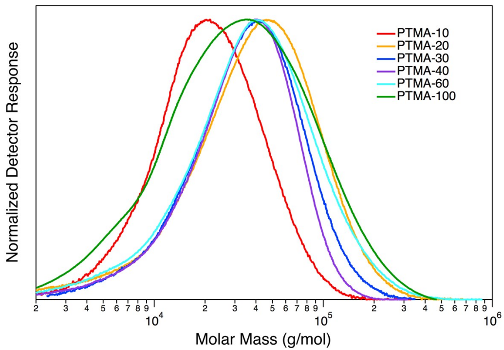
Supplemental Figure S2: GPC traces of PTMA samples.
