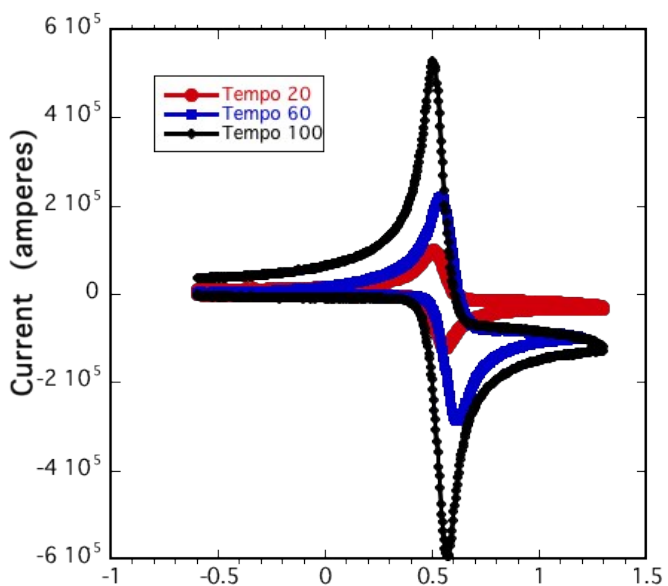
Supplemental Figure S1: Representative CVs of PTMA-20 (red circles), PTMA-60 (blue squares), and PTMA-100 (black diamonds).
