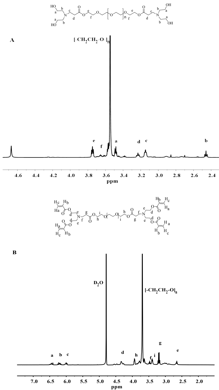
Figure S1 ^1\text{H} NMR spectra of PEG(OH) _4 (A) and PEG(Ac) _4 (B).
