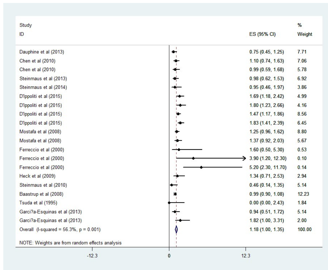
Figure S1 Analysis of the potential lung cancer risks at low to moderate arsenic concentrations.
