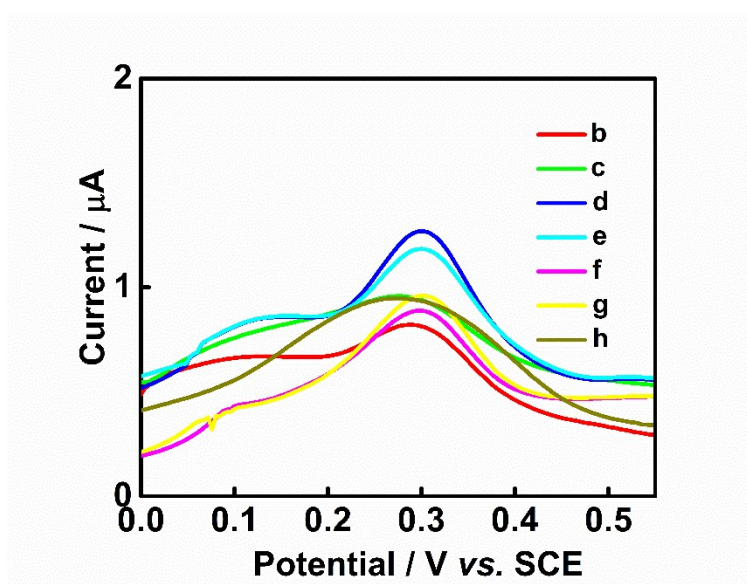
Fig. S1 DPV curves of the modified electrode prepared in the absence of hairpin DNA (b), BPA-aptamer-ssDNA-B (c), \text{CuSO}_4 (d), AA (e), \text{CuBr}_2/\text{Me}_6\text{TREN} (f), PBIB (g) or FMMA (h) in 1 M \text{LiClO}_4 .
