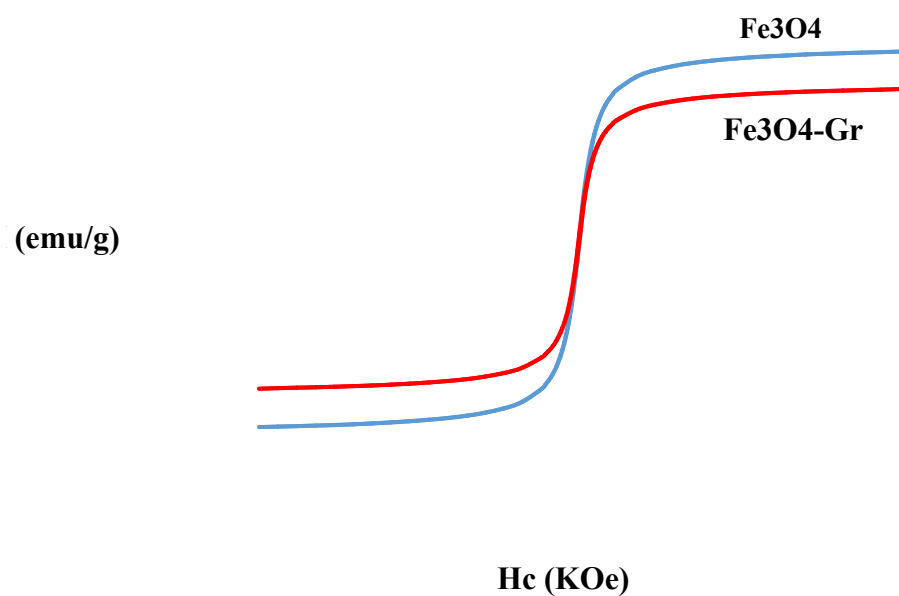
Fig. 1S. VSM magnetization curves of Fe 3 O 4 NPs and (b) Fe 3 O 4 -Gr NPs.
