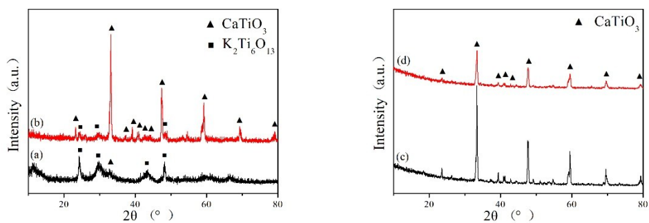
Figure S1. XRD patterns of the sample hydrothermally synthesized under different KOH concentrations and time at 200 °C, (a) 1.0 mol/L KOH, 1 h, (b) 1.0 mol/L KOH, 2 h, (c) 0.25 mol/L KOH, 4 h, (d) 2.0 mol/L KOH, 1h
