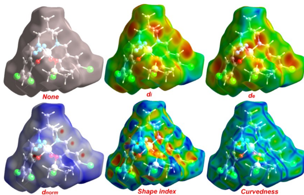
Figure S1: Hirshfeld surfaces of [\text{Co}^{\text{III}}\text{L}^a(\text{N}_3)(\text{DMSO})] , mapped with none, d_i , d_e , d_{\text{norm}} , shape index and curvedness.
