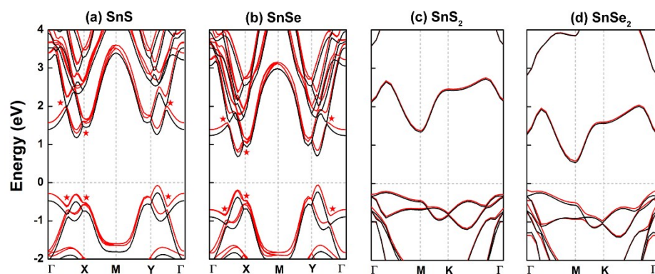
Fig.S1. DFT bandstructure of single-layered SnX and SnX 2 with (red lines) and without SOC (black lines). The red stars represent band splitting on some k points.
