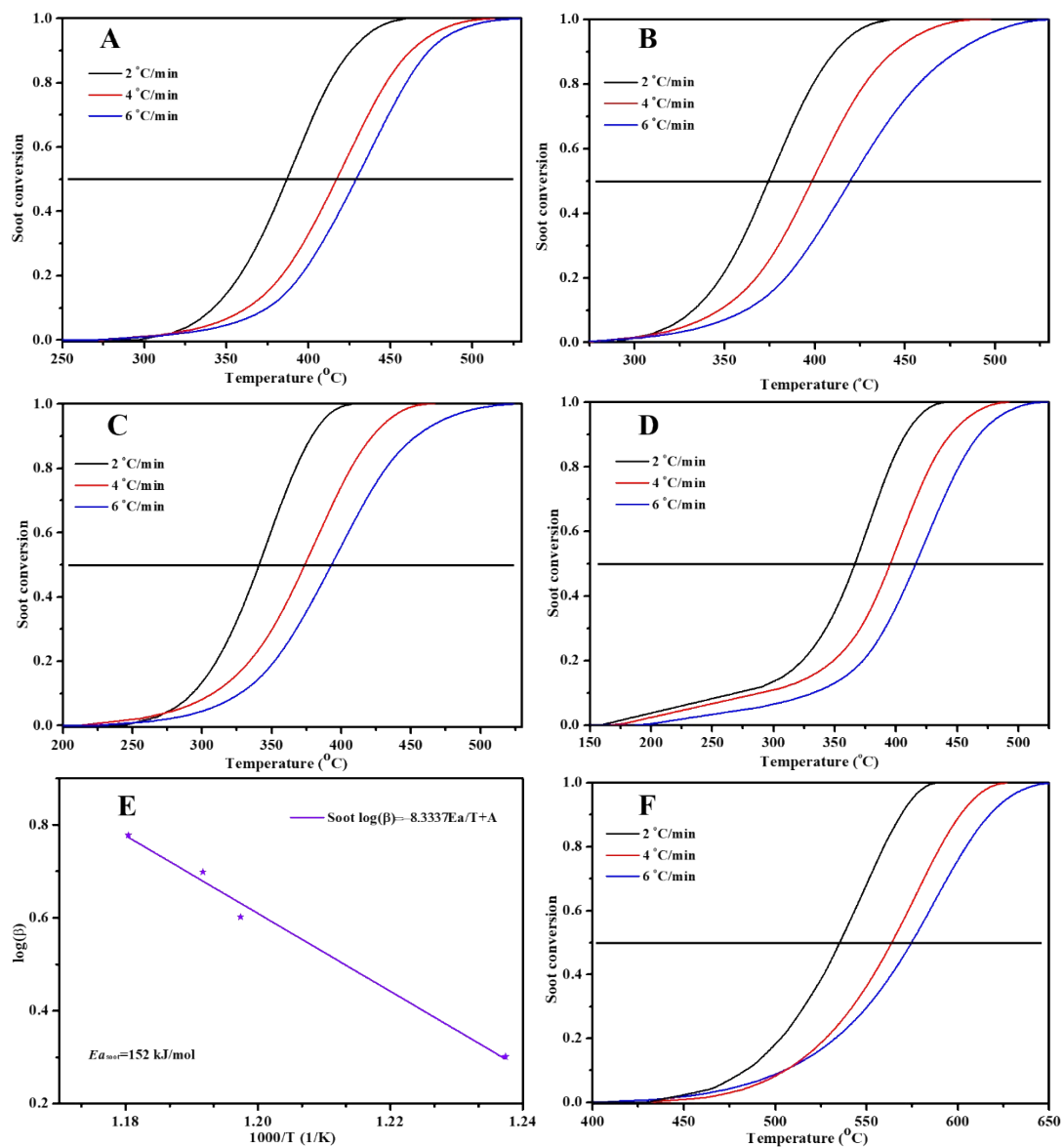
Fig. S2 Detail data of Ozawa method: (A) LSM-0; (B) LSM-1; (C) LSM-3; (D) LSM-5; (E) and (F) pure soot.
