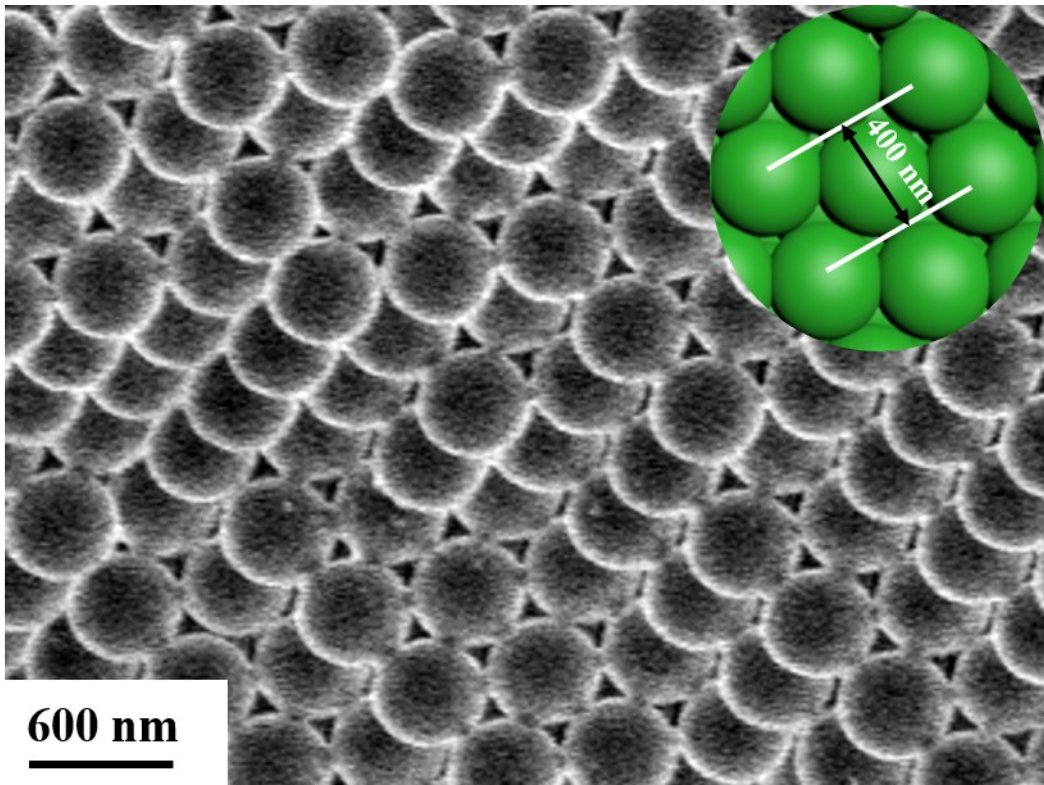
Fig. S1 FESEM images of as-prepared well-packed PMMA microspheres.
