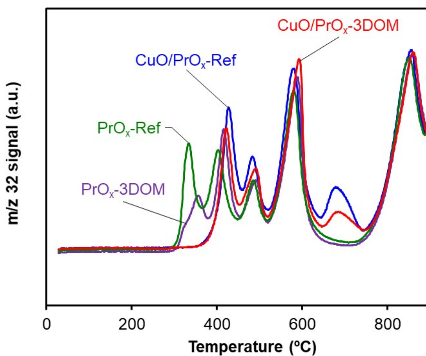
Figure S1. m/z 32 signal evolution during Ar-TPD experiments
