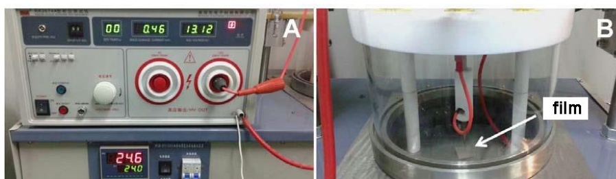
Fig. S1 (A) High voltage supply and (B) the poling equipment, together with a piece of film.
