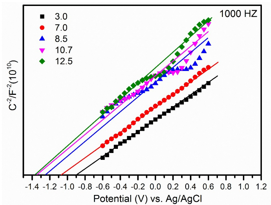
Fig. S1 Typical Mott-Schottky plots of \text{HSr}_2\text{Nb}_3\text{O}_{10} nanosheets in different pH values.
