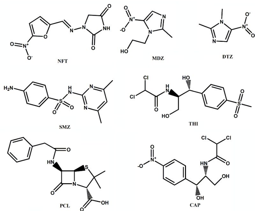
Figure S1. The structures of selected antibiotics.
