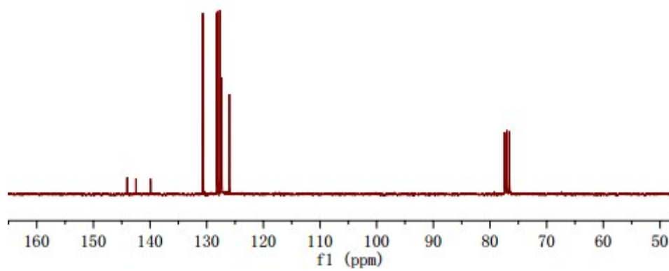
Figure S2 ^{13}\text{C} NMR spectrum of TPD in \text{CDCl}_3
