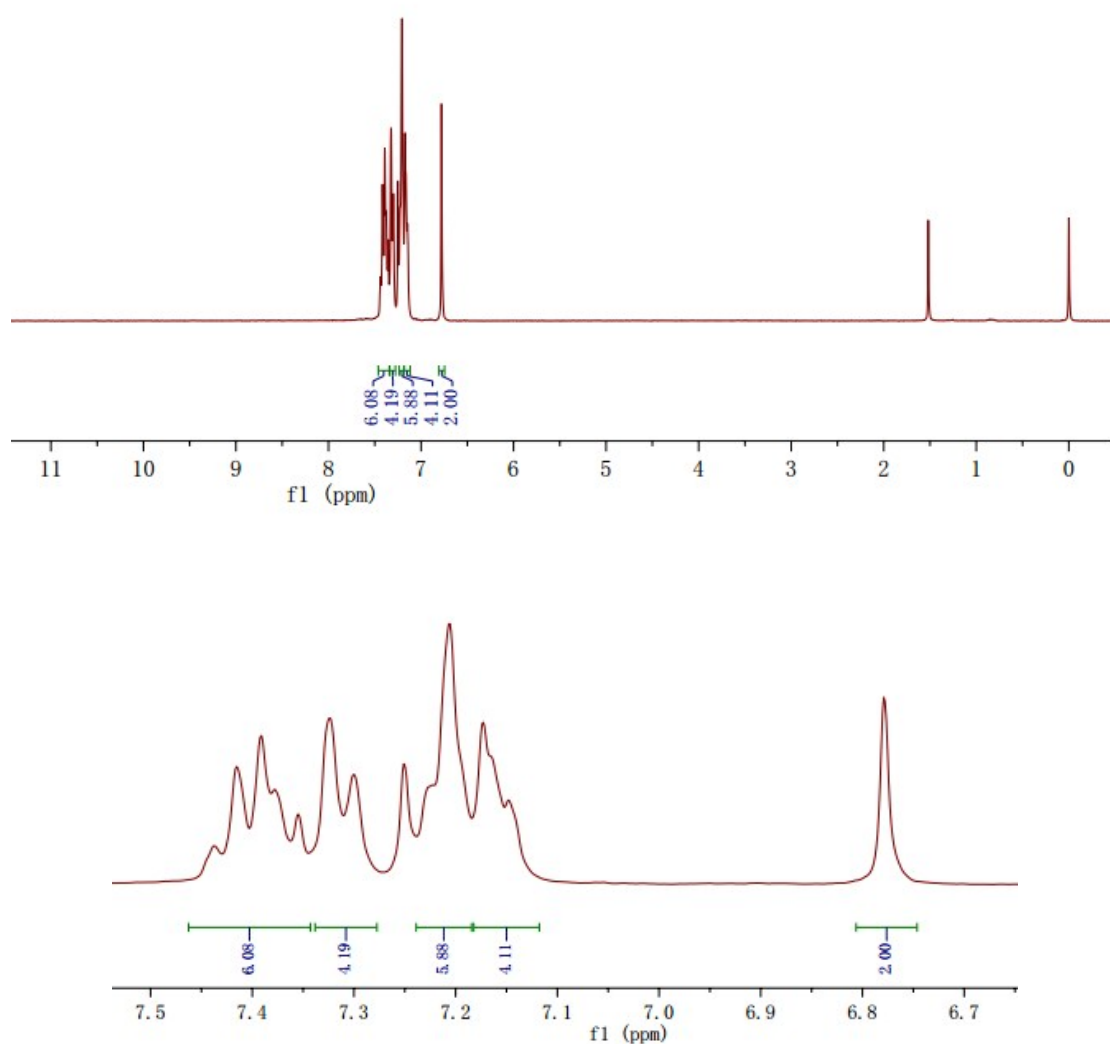
Figure S1 1 H NMR spectrum of TPD in CDCl 3
