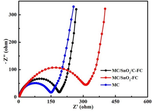
Fig. S2. EIS plots of MC, MC/SnO 2 -FC and MC/SnO 2 /C-FC.
