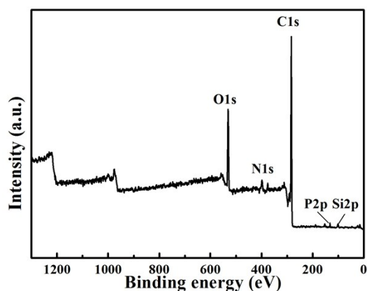
Fig. S1. The XPS results of MC survey scan.
