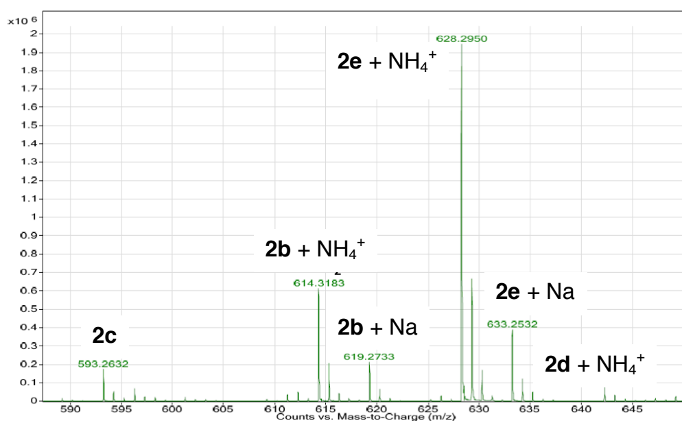
Figure S1. High-resolution electrospray ionization mass spectrum of the crude mixture from the Cannizzaro reaction of 4,4'-diformyldibenzo-30-crown-10 ( 2c ) using NaOH as the base.
