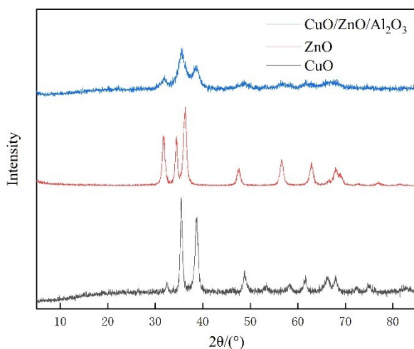
Fig.S1 XRD spectra of CuO, ZnO and CuO/ZnO/Al 2 O 3
