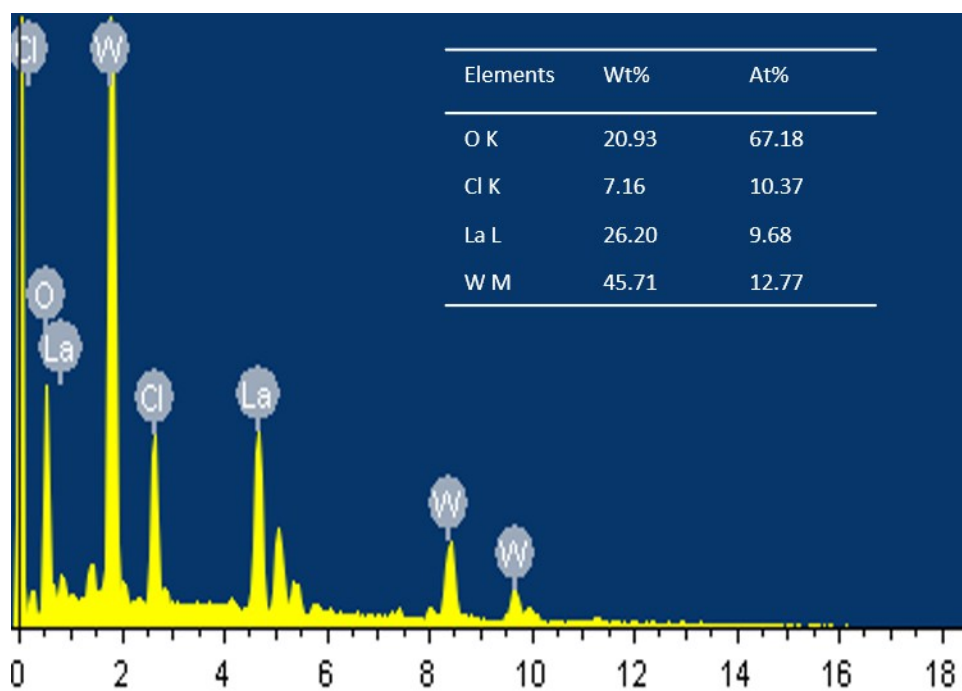
Fig S1 EDS spectrum of the urchin-like \text{LaWO}_4\text{Cl} assemblies
