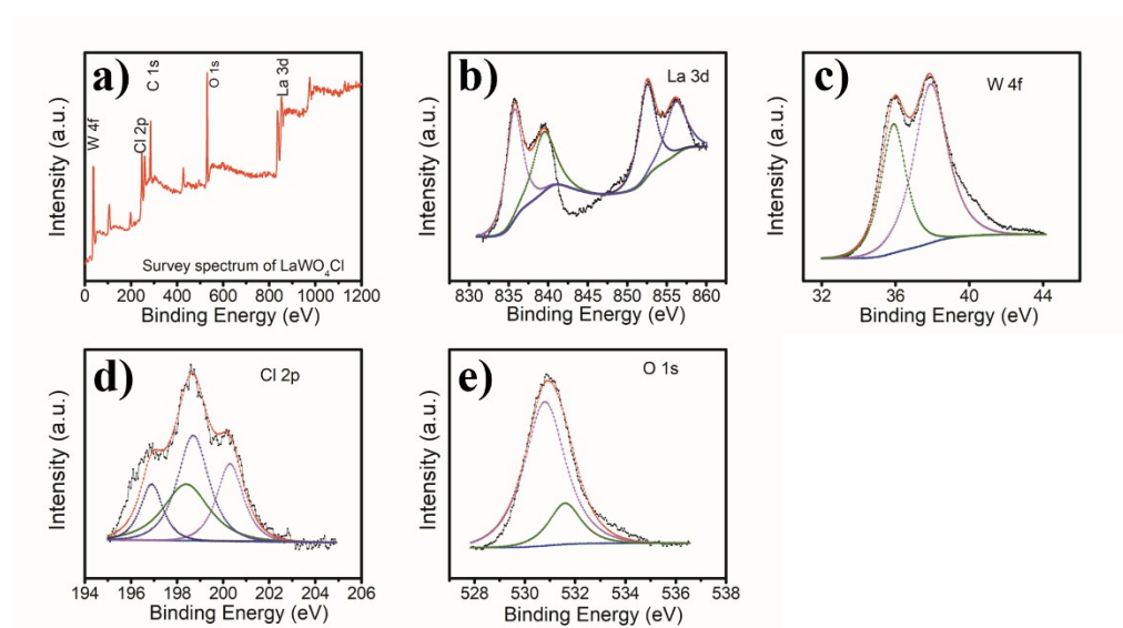
Fig S2 Detailed XPS spectrum of urchin-like \text{LaWO}_4\text{Cl} assemblies
